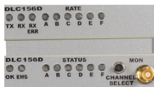
DLC156D front panel monitoring and status display
